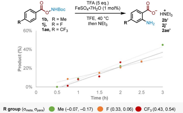
Fig. 2 (A) Reaction order analysis in NaTFA for triflate salt 9a . (B) Rate-determining step (RDS) inference from rate of product formation with varying arene electronics. Yields determined by ^1\text{H} NMR using 1,2-DME as an internal standard after quenching with \text{Et}_3\text{N} and filtering through silica.
