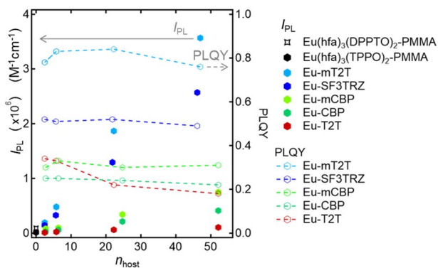
Fig. 4 Host and its ratio dependence of overall luminescence intensities ( I_{PL} ) and PLQY. I_{PL} of the Eu(hfa) 3 (DPPTO) 2 -doped PMMA film (black star marker), Eu(hfa) 3 (TPPO) 2 -doped PMMA film (black hexagon marker), Eu-mT2T film (sky blue hexagon markers), Eu-SF3TRZ film (blue hexagon marker), Eu-mCBP film (yellow green hexagon marker), and Eu-T2T film (red hexagon marker), calculated using eqn (1) and (2). PLQY of the Eu-mT2T film (sky blue line), Eu-SF3TRZ film (blue line), Eu-mCBP film (yellow green line), and Eu-T2T film (red line). n_{\text{host}} is the number of host molecules that contributed to one Eu(III) ion emission.
