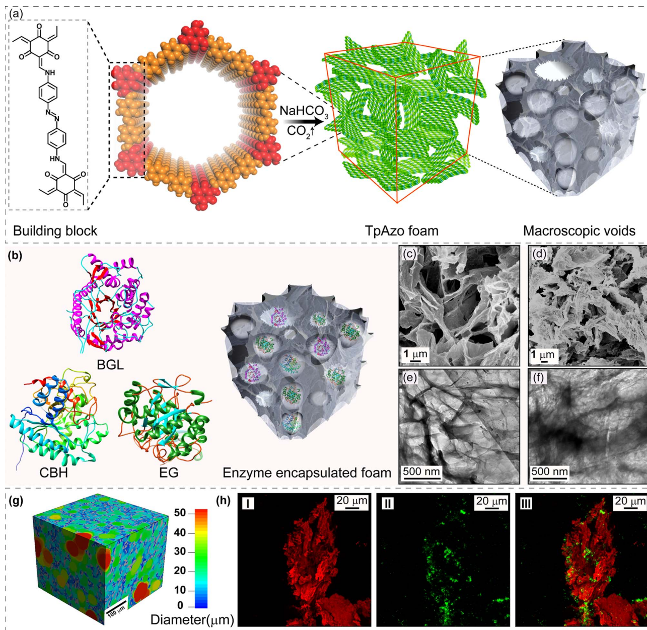
Fig. 1 (a) Schematic representation of the hierarchical TpAZo COF-foam synthesis using an in situ \text{CO}_2 gas-foaming technique. (b) A graphic view of enzymes BGL (β-glucosidase), CBH (cellobiohydrolase), and EG (endoglucanase) immobilized in TpAZo foam with macroscopic voids. SEM images of (c) TpAZo foam and (d) BGL@TpAZo-foam. TEM images of (e) TpAZo foam and (f) BGL@TpAZo-foam. (g) 3D X-ray computed tomographic image of BSA@TpAZo-foam. (h) CLSM image of (I) TpAZo foam (II) FITC-EG immobilized foam (III) overlay image of I and II.
