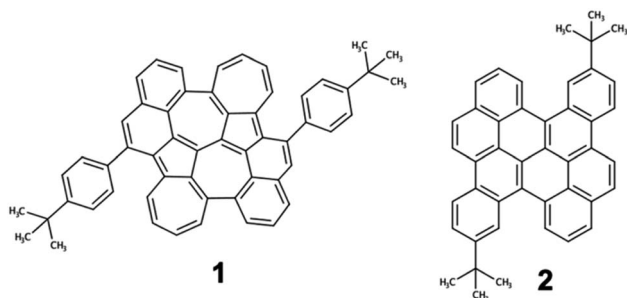
Fig. 5 Molecular structures of diazulenodiazulene[2,1,8- efg :2',1',8'- kla ]heptalene PCH 1 and substituted bischrysenes ( 2 ).
