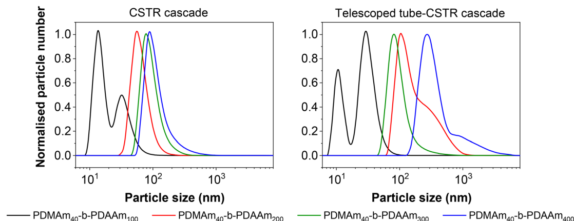
Fig. 10 Particle size distributions of PDMA 40 -b-PDAAm m copolymers prepared via RAFT dispersion polymerisation in a miniature CSTR cascade using a batch macro-CTA (left) versus in a miniature CSTR cascade with a macro-CTA prepared upstream in a telescoped tubular reactor (right). PDMA 40 macro-CTA was prepared at 80 °C for 40 minutes, with copolymerisation at 70 °C for 50 minutes. [CTA] : [initiator] = 10 : 1.
