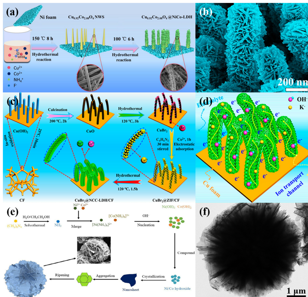
Fig. 6 (a) Synthetic schematic of Cu 0.92 Co 2.08 O 4 @NiCo-LDHs. Adapted with permission from ref. 149 Copyright 2021, Elsevier Ltd. (b) SEM images of the CuBr 2 @NiCeCo-LDH core-shell nanorod, (c) schematic illustration of the CuBr 2 @NiCeCo-LDH core-shell nanorod, and (d) schematic diagram of electron and ion transfer across the surface of the active component. Adapted with permission from ref. 150 Copyright 2022, American Chemical Society. (e) Synthetic schematic of NiCo-LDH synthesis, and (f) TEM image of NiCo-LDHs/S-15. Adapted with permission from ref. 151 Copyright 2022, Elsevier Ltd.
