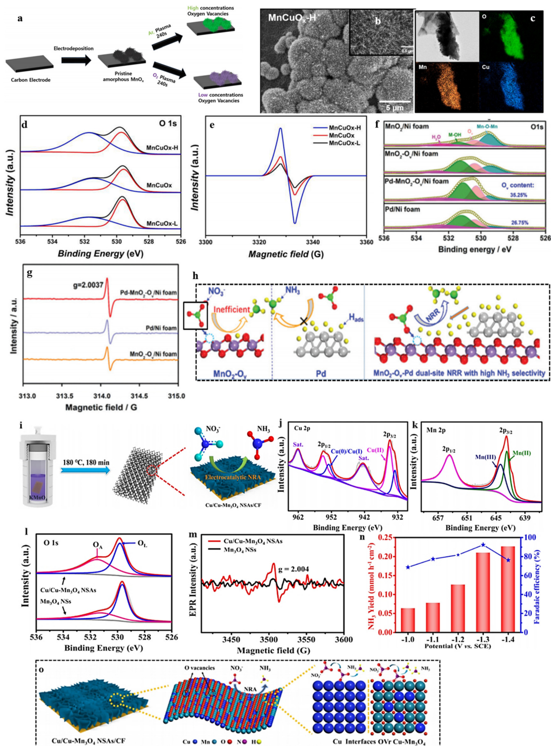
Fig. 20 (a) Illustration in the form of a schematic showing the complete synthesis process for MnCuO x catalysts. (b) SEM morphology of MnCuO x -H. (c) The elemental distribution of oxygen, manganese, copper, and their overlay in a selected area of MnCuO x -H, as shown by EDX. (d and e) The XPS spectra of O 1s and the EPR spectra of the MnCuO x catalysts. Reproduced from ref. 194 with permission from Elsevier, copyright 2023. (f and g) XPS analysis of O 1s of a PdMnO 2 sample and (h) a schematic of the high-NH 3 selectivity MnO 2 -Ov-Pd dual-site NRR mechanism. Reproduced with permission. 195 (i) Electrocatalytic NO 3 - reduction by Cu/Cu-Mn 3 O 4 NSAs/CF: a preparation and illustration scheme. (j-l) XPS spectra of distinct Cu 2p, Mn 2p, and O 1s orbitals in various Cu/Cu-Mn 3 O 4 samples. (m) EPR of Cu/Cu-Mn 3 O 4 samples. (n) Production of NH 3 and FE at different potentials. (o) A schematic representation of the electrocatalytic reduction of NO 3 - to NH 3 conversion on Cu/Cu-Mn 3 O 4 NSAs/CF. Reproduced from ref. 197 with permission from American Chemical Society, copyright 2021.
