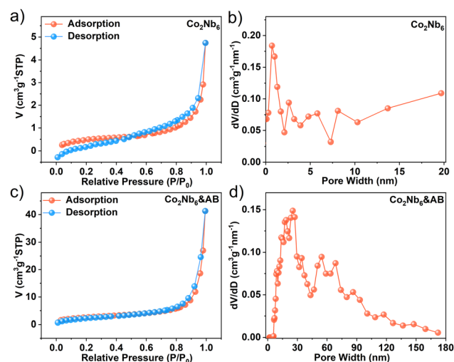
Fig. 4 \text{N}_2 adsorption–desorption isotherms of (a) \text{Co}_2\text{Nb}_6 and (c) \text{Co}_2\text{Nb}_6\&\text{AB} ; and pore size distribution curves for (b) \text{Co}_2\text{Nb}_6 and (d) \text{Co}_2\text{Nb}_6\&\text{AB} .
