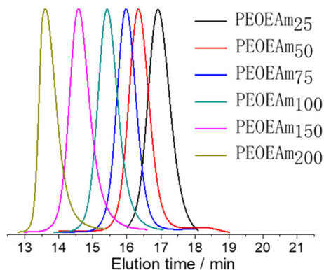
Fig. 1 Size-exclusion chromatography (SEC) traces of PEOEAm obtained by the GTP of EOEAm and \text{Me}_2\text{EtSiH} with [\text{EOEAm}]_0/[\text{Me}_2\text{EtSiH}]_0 ratios of 25, 50, 75, 100, 150, and 200 and with a [\text{Me}_2\text{EtSiH}]_0/[\text{B}(\text{C}_6\text{F}_5)_3]_0 ratio of 0.5.
