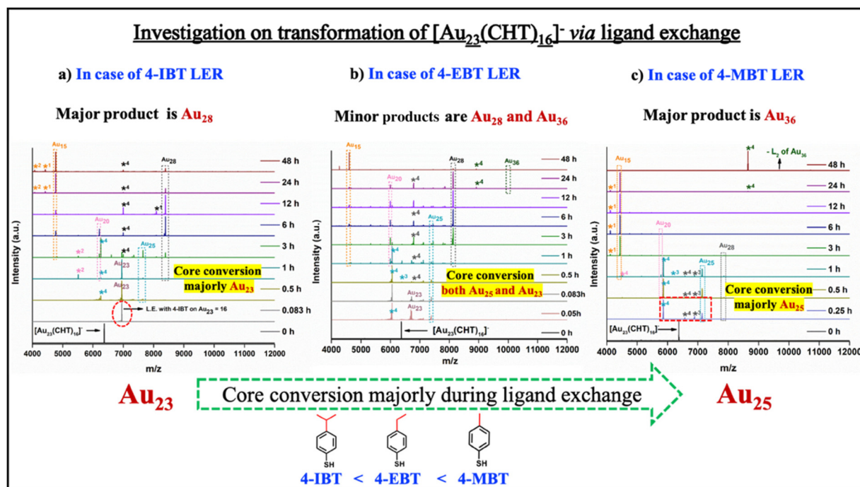
Fig. 3 Time-dependent MALDI-MS spectra showing the transformation process of the [\text{Au}_{23}(\text{CTHT})_{16}]^{-} nanocluster during (a) 4-IBT ligand exchange, (b) 4-EBT ligand exchange, (c) 4-MBT ligand exchange. Note: dark green: \text{Au}_{36} nanocluster and its fragment, cyan: \text{Au}_{25}(\text{SR})_{18} and its fragment, pink: \text{Au}_{20}(\text{SR})_{15} nanocluster and its fragment, orange: \text{Au}_{15} nanocluster and its fragment. SR denotes 4-IBT, 4-EBT, and 4-MBT in the respective spectra. (*) Asterisks represent loss of the AuL fragment where the number with the asterisk represents how many AuL fragments are lost from the respective nanoclusters.
