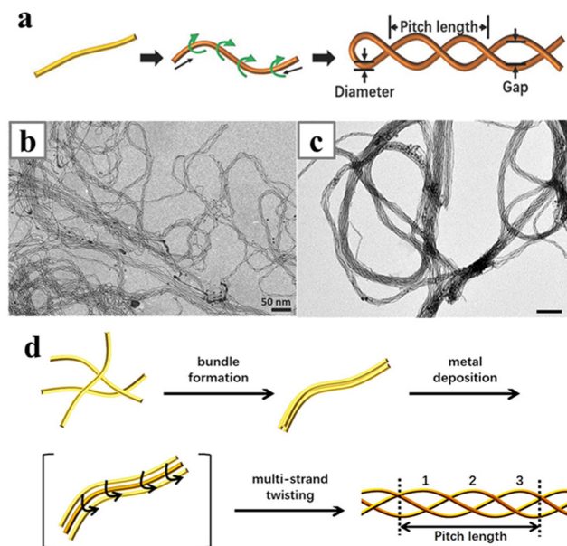
Fig. 20 (a) Schematics illustrating the twisting of Au–Ag double helix nanowires. (b) TEM image of ultrathin Au–Ag alloy helices. (c) TEM image of AuPd nanopores. (d) Schematics illustrating the braiding of AuPd nanopores. Reprinted with permission from ref. 156 and 157. Copyright 2018 from WILEY-VCH GmbH and 2020 from the American Chemical Society.
