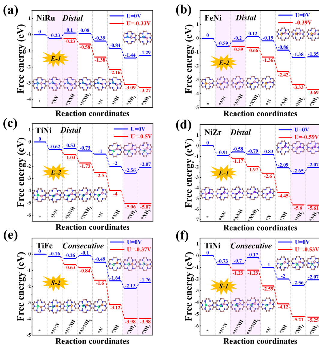
Fig. 5 Free energy diagrams of the NRR on (a) NiRu@C 9 N 4 , (b) FeNi@C 9 N 4 , (c) TiNi@C 9 N 4 and (d) NiZr@C 9 N 4 in the distal mechanism, (e) TiFe@C 9 N 4 and (f) TiNi@C 9 N 4 in the consecutive mechanism. Blue and red lines indicate free energy changes for the NRR at U = 0 V and U_L , respectively.
