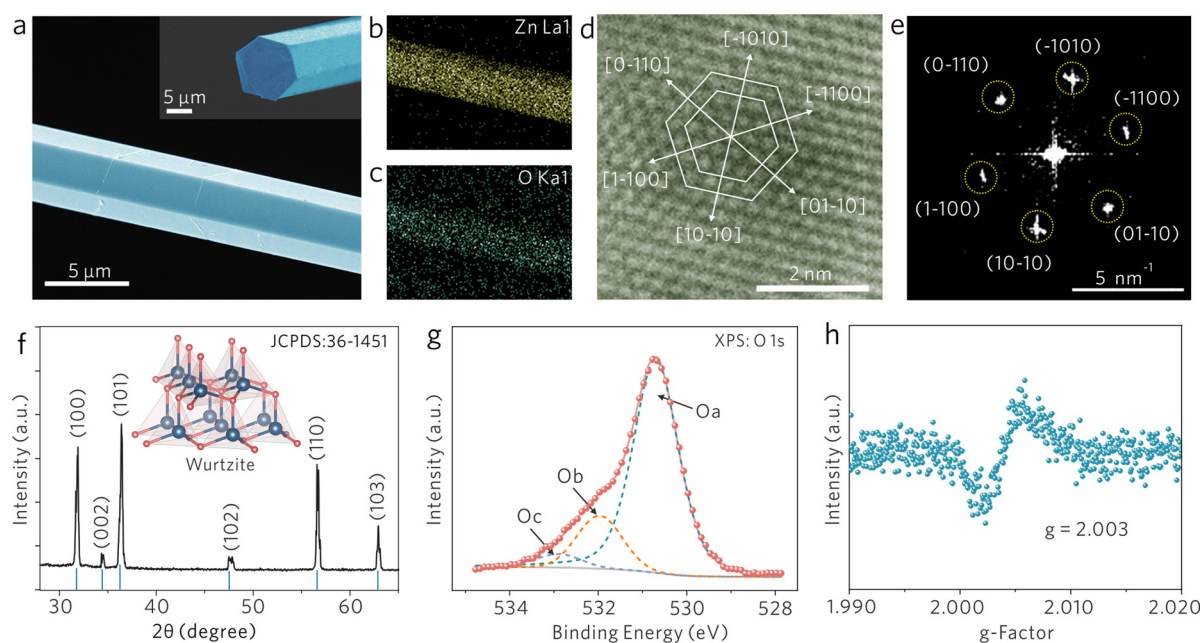
Fig. 1 Characterization of the \text{ZnO}_{1-x} WGM cavity. (a) SEM image of the \text{ZnO}_{1-x} cavity. Inset: the hexagonal cross-section of the \text{ZnO}_{1-x} cavity. (b and c) Elemental mapping images of Zn and O of the \text{ZnO}_{1-x} cavity shown in (a). (d) HR-TEM image and the corresponding (e) SAED patterns of \text{ZnO}_{1-x} . (f) XRD and (g) XPS spectrum of the \text{ZnO}_{1-x} cavity. (h) EPR spectrum of the \text{ZnO}_{1-x} cavity.
