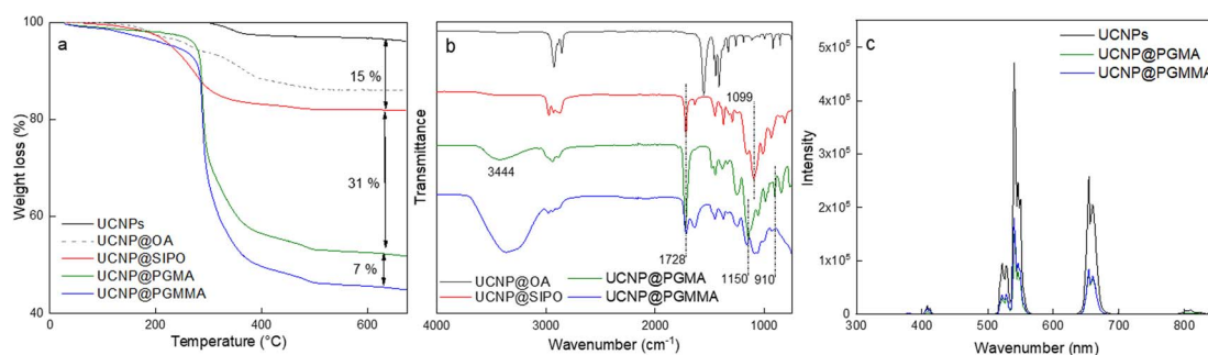
Fig. 3 (a) TGA thermograms, (b) FTIR spectra and (c) fluorescence emission spectra of UCNPs, UCNPs@OA, UCNPs@SIPO, UCNPs@PGMMA, and UCNPs@PGMA particles. UCNPs@SIPO = 3 w/w; UCNPs@GMA = 0.5 w/w.
