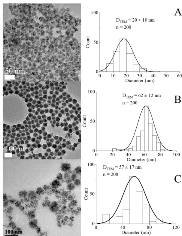
Fig. 3 TEM images and histograms for D_{\text{TEM}} of NFs prepared from [\text{Mn}(\text{acac})_3]/[\text{Fe}(\text{acac})_3] = (A) 1 and (B) 3, respectively at 200 °C, (C) ratio = 7 at 250 °C.
