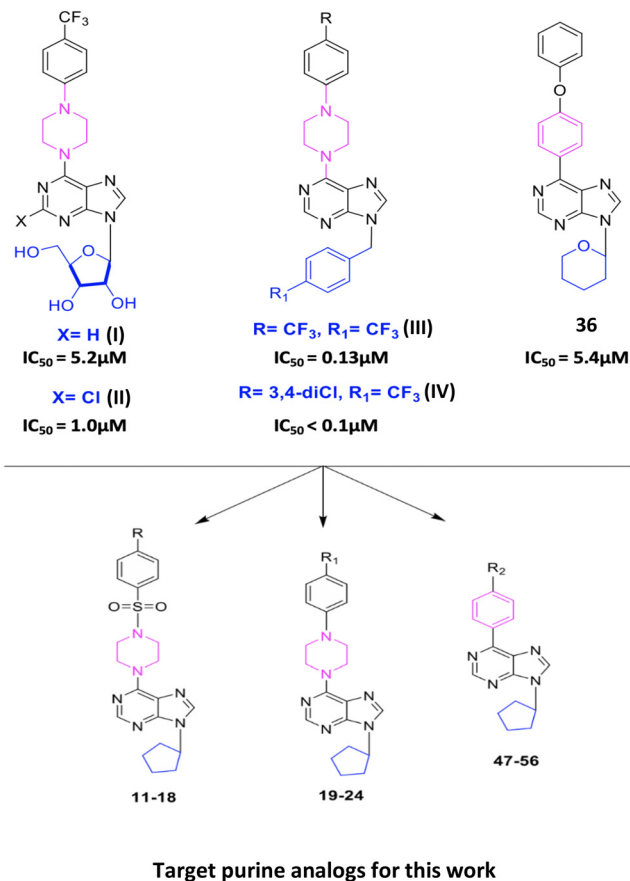
Fig. 1 Structures of 9-(β-D-ribofuranosyl)/4-trifluoromethyl/4-chlorobenzyl/tetrahydropyran)-6-(4-trifluoromethylphenyl)piperazine/4-phenoxyphenyl) purine analogs (I), (II), (III), (IV), and 36 and target purine compounds 11–24 and 47–56.
