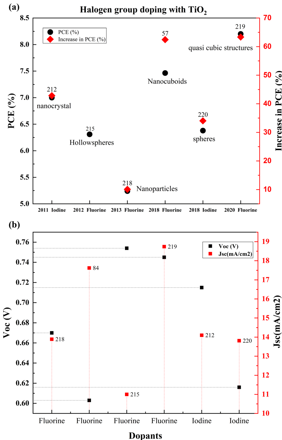
Fig. 25 (a) Comparison of the PCEs of different halogen doped \text{TiO}_2 based DSSCs from 2011. (b) J_{sc} and V_{oc} of halogen doped \text{TiO}_2 based DSSCs. Data points are labelled with references.
