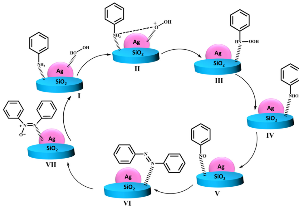
Scheme 9 Schematic illustration of the mechanism during the oxidation of aniline to azoxybenzene.
