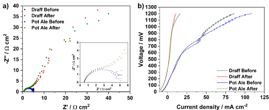
Fig. 12 Complex-plane EIS for PEMEC2 operating with digested draff (D4)–PMA and pot ale (PA2)–PMA analyte solutions, collected at 850 mV before and after chronoamperometry experiments, and (b) V – I curves for PEMEC2 operating with the same analyte solutions, before and after chronoamperometry experiments at 80 °C using \text{H}_2\text{SO}_4 as a catholyte.
