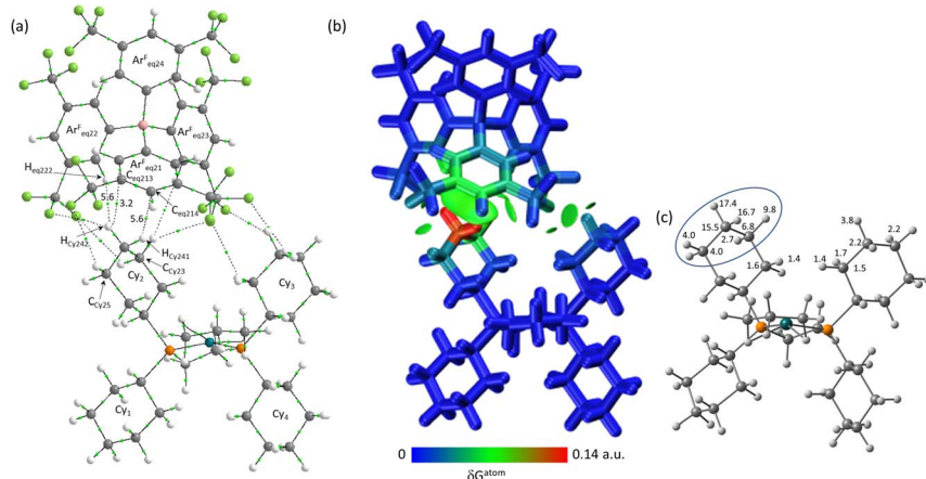
Fig. 8 (a) QTAIM molecular graph with Eq-2 in [\text{1-propane}][\text{BAR}^{\text{F}}_4] with BCPs in green and showing selected atoms and BCP electron densities (a.u. \times 10^{-3} ). Bond paths with \rho(r) < 0.001 a.u., intramolecular bond paths and ring critical points (RCP) are omitted for clarity. (b) IGMH plot where the cation and anion are defined as separate fragments. \text{Sign}(\lambda_2)\rho -coloured isosurfaces are plotted with \delta G^{\text{inter}} = 0.003 a.u. and atoms are coloured by \delta G^{\text{atom}} . (c) \% \delta G^{\text{atom}} contributions on the cation that are above 1%, with the propylene motif highlighted (see text for details).
