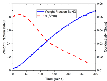
Fig. 10 Trend in calculated conductivity and phase fraction of BaND for doping of \text{BaD}_2 with \text{N}_2 experimentally. The emergence of BaND is associated with a decrease in conductivity. Beyond 280 min, the resistance associated with the high frequency response increases dramatically making the accurate modelling of the R_s difficult.
