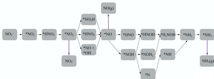
Fig. 2 Reaction paths and possible intermediates for the electrochemical reduction of \text{NO}_3^- to \text{NH}_3 are considered in this work. Magenta arrows indicate the formation of nitric oxide (NO), nitrite ( \text{NO}_2^- ), and ammonia ( \text{NH}_3(\text{g}) ). The dashed arrow indicates a reaction with a proton transfer, and the solid arrows indicate reactions with a proton/electron pair transfer.
