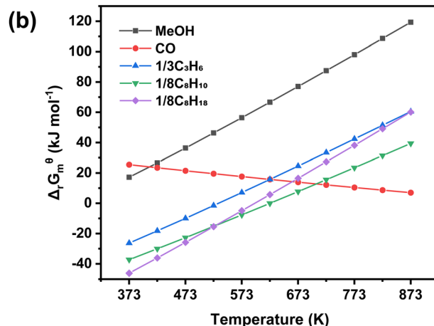
Fig. 3 Thermodynamics analysis. (a) Equilibrium conversion and selectivity in CO 2 hydrogenation to methanol and CO, (b) Gibbs free energy of CO 2 hydrogenation to different products.
