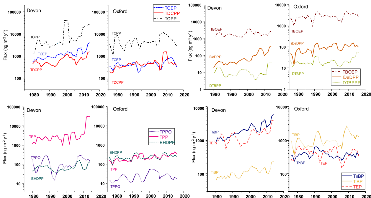
Fig. 3 OPEs fluxes (ng m -2 y -1 ) in Devon Ice Cap (1979–2014) and Mt. Oxford icefield (1975–2016).
