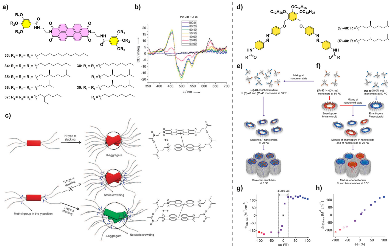
Fig. 20 (a) Chemical structure of PDIs 33 – 39 . (b) CD spectra of mixtures of PDIs 33 and 35 at different ratios ( c_T = 10 \mu\text{M} in MCH/CHCl 3 80/20). (c) Schematic representation of the polymerization of PBIs 33 – 39 into H- or J-aggregates (reproduced from ref. 92 with permission from Wiley-VCH, copyright 2008). (d) Chemical structure of (S)- and (R)- 40 . (e) and (f) Schematic representations of the distinct hierarchical organization of (S)- 40 and (R)- 40 . (g) MR experiment performed in scalmic nanotoroids as prepared in (e). (h) MR experiment performed in mixtures of enantiopure nanotubes as prepared in (f) ( c_T = 300 \mu\text{M} in MCH) (reproduced from ref. 96 with permission from the American Chemical Society, copyright 2023).
