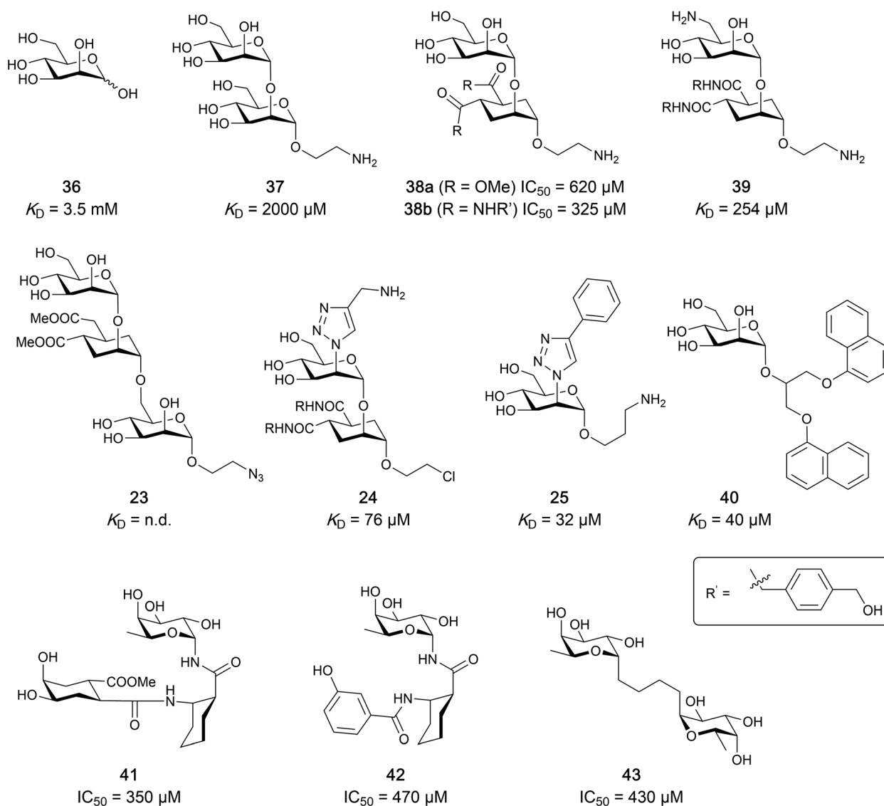
Fig. 8 Carbohydrate-based glycomimetic DC-SIGN inhibitors. The ligands are derivatives of mannose ( 25 , 40 ), manno- and fucosylated disaccharides ( 24 , 37–39 ) and mannotriose ( 23 ) and fucose ( 41–43 ).
