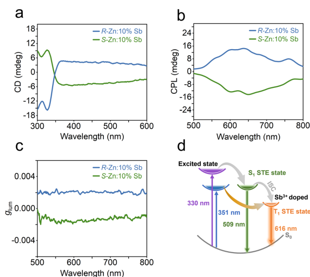
Fig. 4 (a) CD spectra, (b) CPL spectra and (c) corresponding g_{\text{lum}} of \text{R-/S-Zn}:10\%\text{Sb} . (d) Schematic illustration of the proposed PL process in \text{R-Zn}:x\%\text{Sb} .
