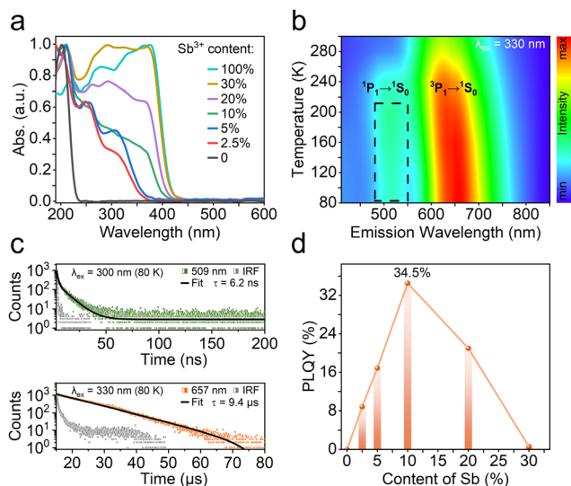
Fig. 3 (a) UV-vis absorption spectra, (b) varied-temperature PL spectra of \text{R-Zn}:10\%\text{Sb} at excitation of 330 nm, (c) PL decay profiles of 509 and 657 nm at 80 K for \text{R-Zn}:10\%\text{Sb} , and (d) quantum yield of \text{R-Zn}:x\%\text{Sb} with various \text{Sb}^{3+} dopant amounts.
