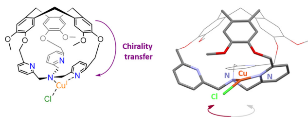
Fig. 11 Schematic representation of the chirality transfer observed in \text{M-Cu}^{\text{I}}(\text{Hm-CH}_2\text{-TPA})(\text{Cl}) (left), along with view of its XRD structure (right).
