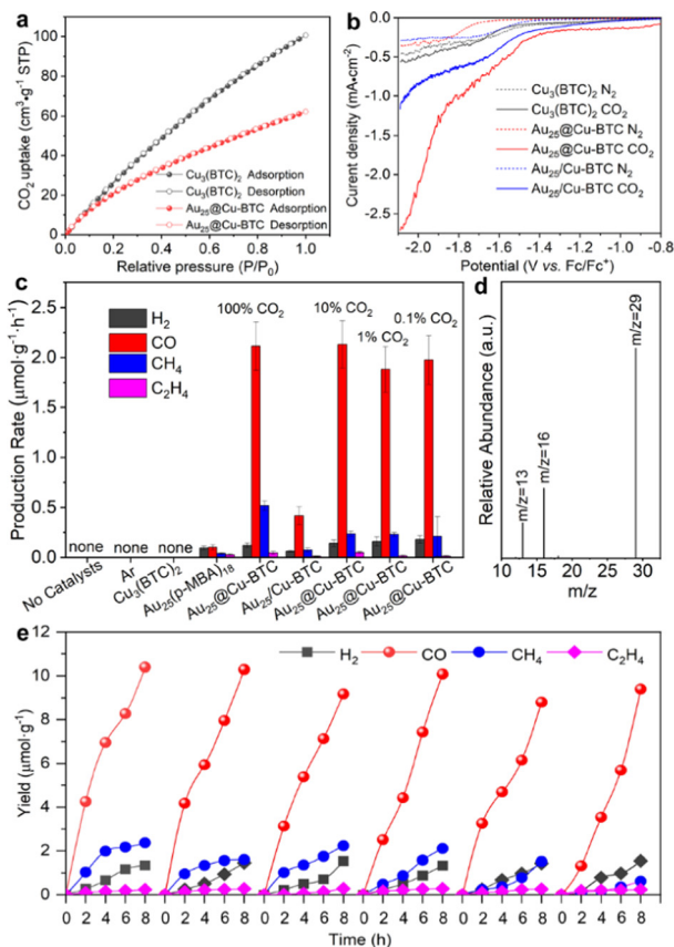
Fig. 2 (a) \text{CO}_2 adsorption behavior for \text{Au}_{25} @Cu-BTC and bare \text{Cu}_3(\text{BTC})_2 . (b) LSV curves of pristine \text{Cu}_3(\text{BTC})_2 , \text{Au}_{25} @Cu-BTC and mechanically mixed \text{Au}_{25}/\text{Cu-BTC} in 0.1 M TBAHFP solution saturated with \text{N}_2 or \text{CO}_2 . (c) Average production rates of \text{H}_2 , \text{CO} , \text{CH}_4 and \text{C}_2\text{H}_4 in photoreduction \text{CO}_2 by \text{Au}_{25} @Cu-BTC in the first 2 h under visible-light ( \lambda > 420 nm) irradiation, in comparison with those by \text{Cu}_3(\text{BTC})_2 , \text{Au}_{25}(\text{p-MBA})_{18} , \text{Au}_{25}/\text{Cu-BTC} and other control experiments under the same conditions. All measurements were performed on a gas–solid reactor in the presence of BIH and a trace amount of \text{H}_2\text{O} . (d) GC–MS analysis of ^{13}\text{CO} ( m/z = 29 ) produced over \text{Au}_{25} @Cu-BTC in light-driven reduction of ^{13}\text{CO}_2 . (e) Light-driven catalytic durability over \text{Au}_{25} @Cu-BTC. Each cycle takes 8 h.
