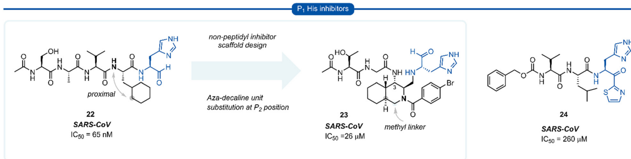
Fig. 6 Representative examples of P 1 His inhibitors targeting SARS-CoV 3CL pro .
