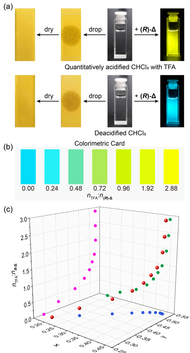
Fig. 4 Detecting traces of acids employing (R)-Δ . (a) Fluorescence changes of solutions (right) of (R)-Δ in \text{CHCl}_3 with and without TFA upon shining 365 nm-UV light in comparison with detecting trace acid in the same solvents using pH papers (left). (b) A colorimetric card showing the ability of (R)-Δ to detect visually amounts of acid in solutions with different n_{\text{TFA}}:n_{(\text{R})-\Delta} ratios. (c) The fitting function based on the PL emission of (R)-Δ upon changing the n_{\text{TFA}}:n_{(\text{R})-\Delta} ratio from 0.00 to 2.88. The concentration of (R)-Δ is 1 \times 10^{-5} M.
