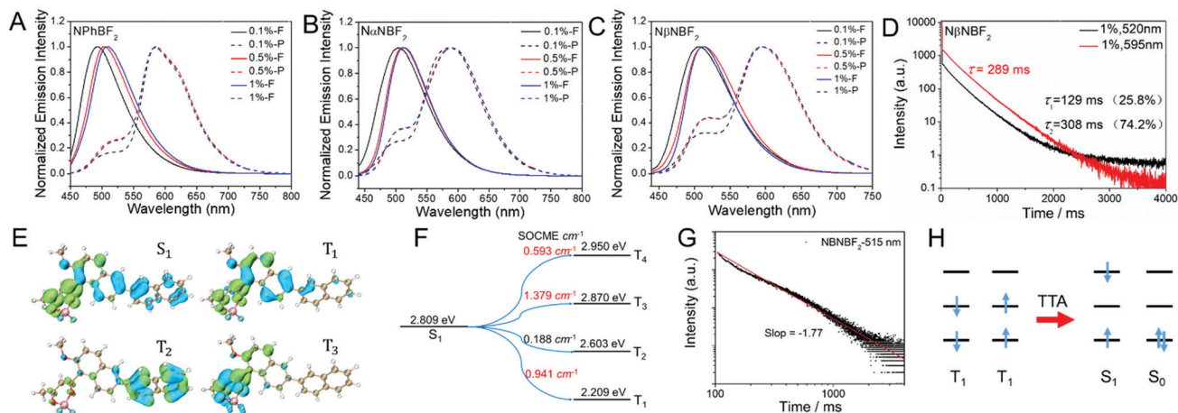
Fig. 3 (A–C) The room-temperature emission spectra collected in fluorescence mode and phosphorescence mode (1 ms delay) of (A) NPhBF 2 -MeOBP, (B) NaNBF 2 -MeOBP and (C) NβNBF 2 -MeOBP afterglow materials with weight ratios fixed at 0.1%, 0.5% and 1%, respectively. The spectra collected in fluorescence mode denote steady-state emission spectra. The spectra collected in phosphorescence mode represent delayed emission spectra that contain both phosphorescence and delayed fluorescence. (D) The room-temperature emission decay of NβNBF 2 -MeOBP-1% afterglow materials monitored at 520 nm and 595 nm, respectively. (E) The isosurface maps of NβNBF 2 singlet and triplet excited states based on the TD-DFT calculated results. Blue and green isosurfaces correspond to hole and electron distributions, respectively. (F) TD-DFT calculated energy levels of NβNBF 2 singlet and triplet excited states and their spin-orbit coupling matrix elements (SOCME). (G) The double logarithmic plot of the room-temperature emission decay profile of NβNBF 2 -MeOBP-0.5% afterglow materials monitored at 515 nm. (H) Schematic illustration of the TTA mechanism.
