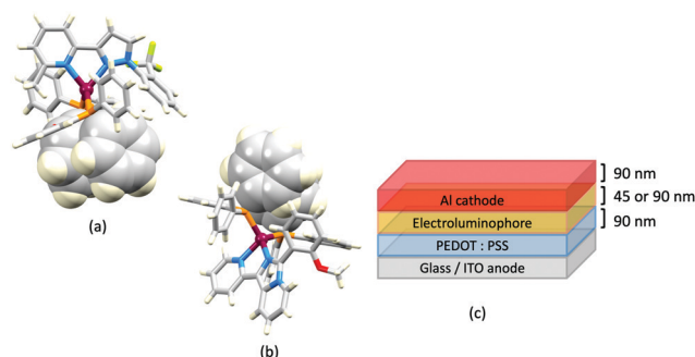
Fig. 16 Structures of the complex cations in (a) [Cu(POP)( 8 )] + [BF 4 ] − ·EtOH (CSD refcode JUFNOP) and (b) [Cu(POP)( 11 )] + [PF 6 ] − showing Ph-arene \pi -stacking in the POP ligand (space-filling representation). (c) LEC architecture for testing with [Cu(POP)( 11 )] + [PF 6 ] − in the active layer; LECs were driven with a pulsed current.
