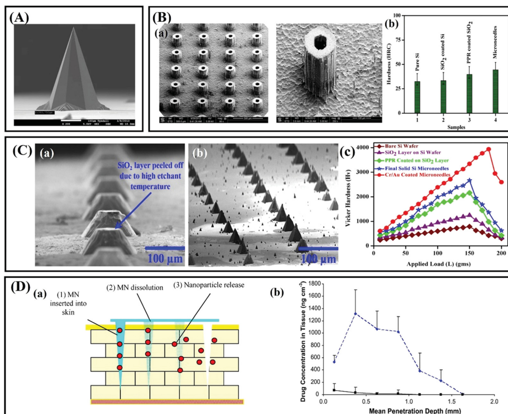
Fig. 3 (A) Solid silicon MNs (height: \sim 400 \mu\text{m} ). Adapted with permission from ref. 34. Copyright 2014 Springer Nature. (B) (a) SEM image of hollow silicon MNs. (b) Vickers hardness test measured and compared for solid Si MNs. Adapted with permission from ref. 27. Copyright 2014 Elsevier. (C) (a) Single row of MNs with the \text{SiO}_2 layer peeled off. (b) Final high aspect ratio of solid Si MNs. (c) Measured and compared-load versus Vickers hardness (Hv) values for all samples. Adapted with permission from ref. 36. Copyright 2018 Springer Nature. (D) (a) Schematic representation of the steps involved in Nile Red release from the polymeric MN system. (b) The concentration of Nile Red in excised neonatal porcine skin following the application of PMVE/MA MNs containing Nile Red-loaded nanoparticles and control patches containing Nile red nanoparticles. Adapted with permission from ref. 39. Copyright 2010 Elsevier.
