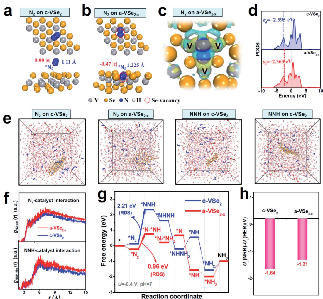
Fig. 4 (a and b) Optimized structures of *N_2 on c-VSe 2 and a-VSe 2-x . (c) Electron deformation density of *N_2 on a-VSe 2-x . Yellow and cyan iso-surfaces represent electron accumulation and electron depletion, respectively. (d) PDOS of V-3d in c-VSe 2 and a-VSe 2-x for determining the d-band center ( \epsilon_d ). (e) Snapshots of the dynamic process of N 2 /NNH adsorption on c-VSe 2 and a-VSe 2-x in LiClO 4 electrolyte after 5 ns MD simulations, and corresponding (f) RDF curves of N 2 -catalyst and NNH-catalyst interactions. (g) Free energy diagrams of energetically favorable NRR pathways on c-VSe 2 and a-VSe 2-x at U = -0.4 V and \text{pH} = 7 . (h) U_L(\text{NRR}) - U_L(\text{HER}) of c-VSe 2 and a-VSe 2-x .
