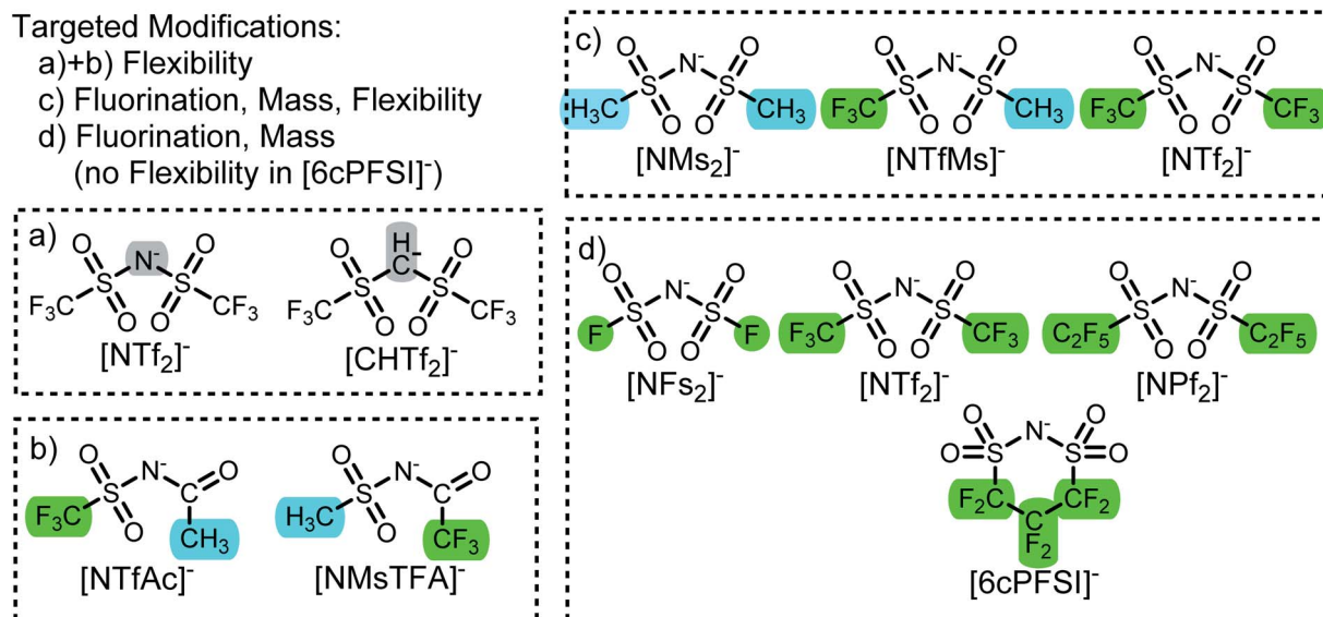
Fig. 2 Targeted modifications of the [NTf_2]^- anion investigated in this work. Tf = triflate, Ac = acetyl, TFA = trifluoroacetyl, Ms = methanesulfonyl, FS = fluorosulfonyl, Pf = pentafluoroethylsulfonyl.
