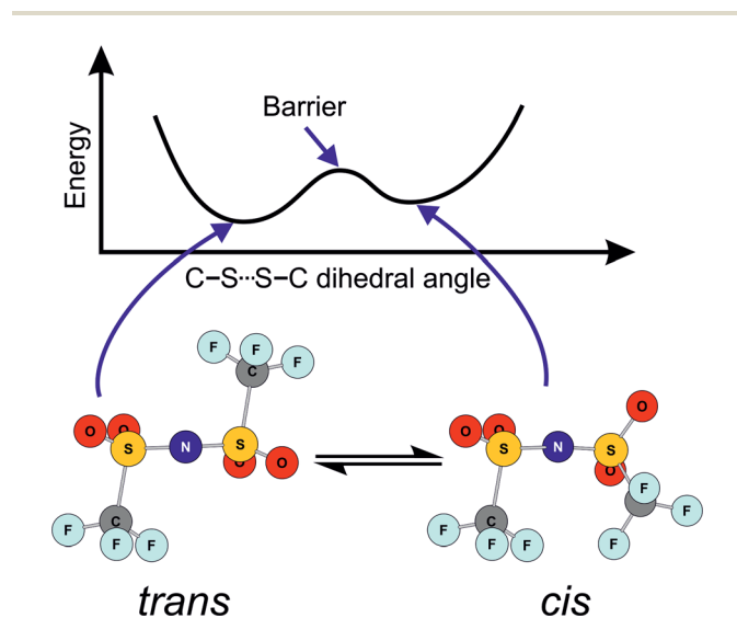
Fig. 1 Schematic of the two minimum energy conformers of the [\text{NTf}_2]^- anion, and of the energy as a function of the C–S...S–C dihedral angle. Adapted from ref. 39.
