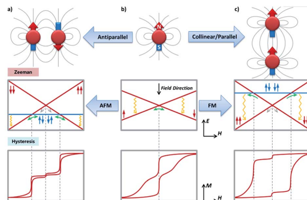
Fig. 4 The dipolar couplings between two neighbouring spin centres with strong axial anisotropy, showing the importance of the relative orientation of the magnetic moments with their spatial locations (top), from an independent spin center (b) to a ferromagnetic (c) or anti-ferromagnetic (a) dimer. The solid grey lines qualitatively represent the magnetic field lines generated by the spin centre treated as a small bar magnet. The corresponding Zeeman diagrams (middle) and the typical magnetic hysteresis loops (bottom, at a relatively low temperature) are also presented. Green/grey arrows indicate the possible positions for strong/weak avoided level crossings and thus fast/slow QTM, respectively. They are further linked with the steps on the magnetic hysteresis loops by the grey dashed lines. The one-way green arrows in the FM scenario should be particularly noted, which only happens in the demagnetization process. Field-enhanced relaxation process such as the direct process is mainly responsible for the closing of the hysteresis loops at higher fields, which is marked with yellow wavy arrows.
