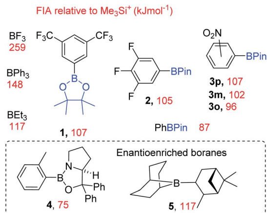
Fig. 3 Boranes employed as phase transfer catalysts in this study and their respective calculated (at the DSD-BLYP-D3(BJ)/def2TZVP level with SMD CH 2 Cl 2 ) fluoride ion affinity (FIA, red). 3o, 3m and 3p = the ortho , meta and para isomers.
