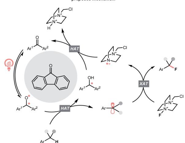
Scheme 10 Ketone-catalysed \text{C}(\text{sp}^3)\text{-H} fluorination.
