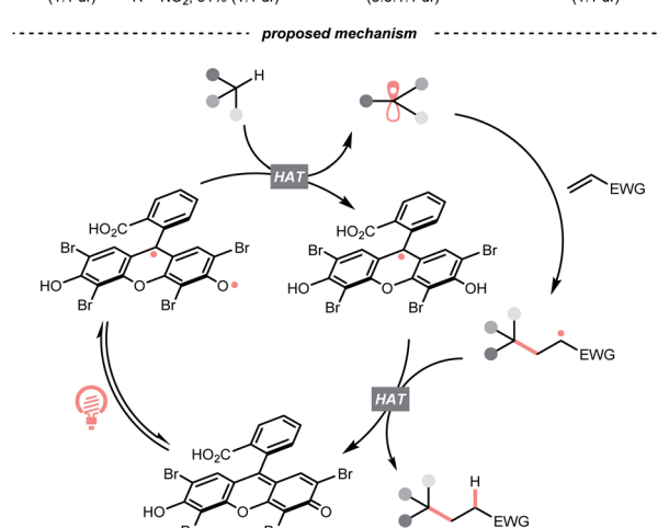
Scheme 11 Eosin Y-catalysed \text{C}(\text{sp}^3) radical generation.
