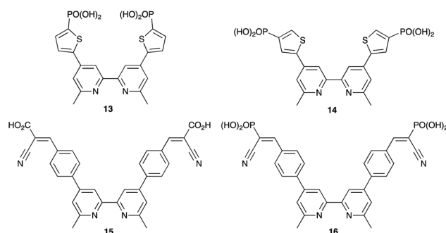
Scheme 17 Structures of some anchoring ligands used with heteroleptic copper(II) dyes. See also Scheme 15.
