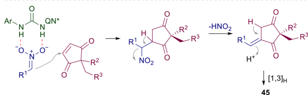
Scheme 33 Alkylation of cyclopent-2-en-1-one derivatives catalyzed by quinone-derived chiral urea 44 .
