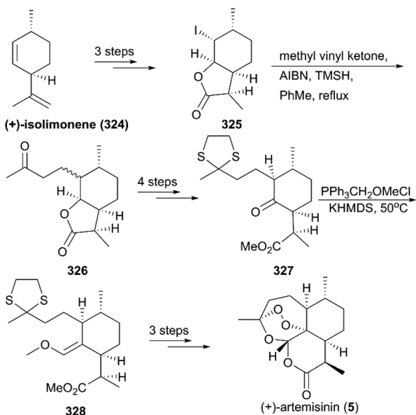
Scheme 35 Total synthesis of (+)-artemisinin by Yadav.
