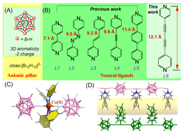
Fig. 1 (A and B) Structure of \text{closo-}[B_{12}H_{12}]^{2-} and organic ligands. (C) General coordination mode in BSFs. (D) General 1D pore channels of interpenetrated BSFs.
