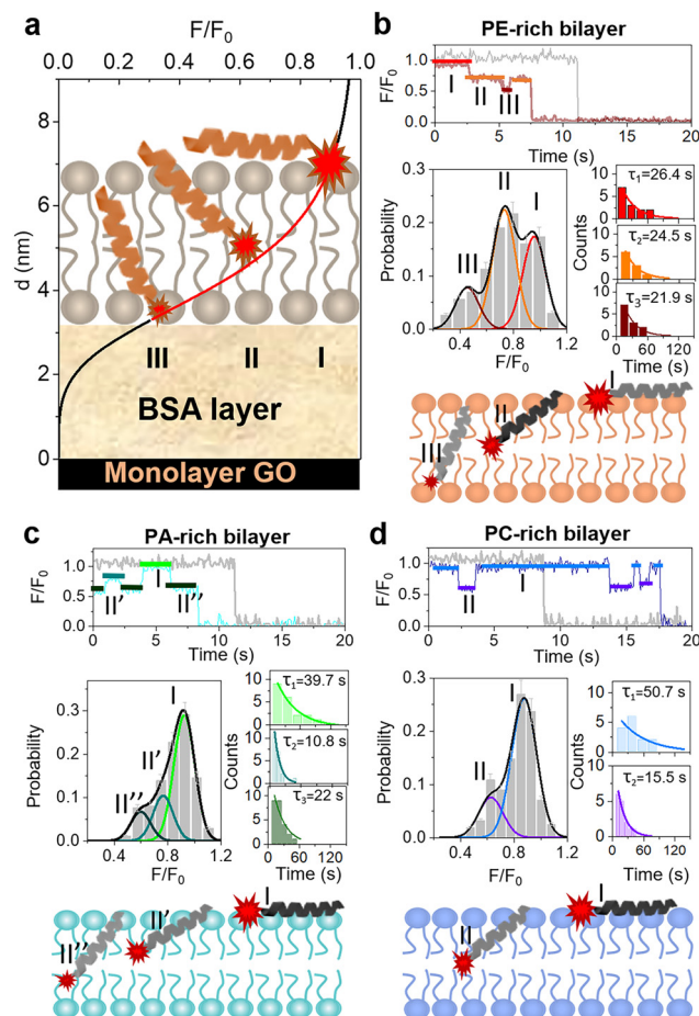
Fig. 2 Dynamics of monomeric LL-37 insertion in different lipid bilayers. (a) Schematic illustration of the single-molecule SIFA method. (b–d) Dynamics of N-TAMRA-LL-37 insertion into (b) PE-, (c) PA-, and (d) PC-rich SLB membranes. The top graph shows a representative normalized fluorescence intensity trace of peptides. Colored straight lines are step fits of the trace. A reference molecule (on the substrate region without GO) is also shown in gray. The graph in the middle-left shows fluorescence intensity distributions analyzed based on around 200 traces each. The colored lines represent fitting curves and were used to determine the states. The middle-right graph shows the dwell times of different states. The bottom graph shows configurational cartoons of the mean position of fluorescence-labeled N-terminus LL-37 peptides corresponding to each state in the membrane. The data were collected immediately after LL-37 addition. I, II (II' or II''), and III represent different states in the bilayer.
