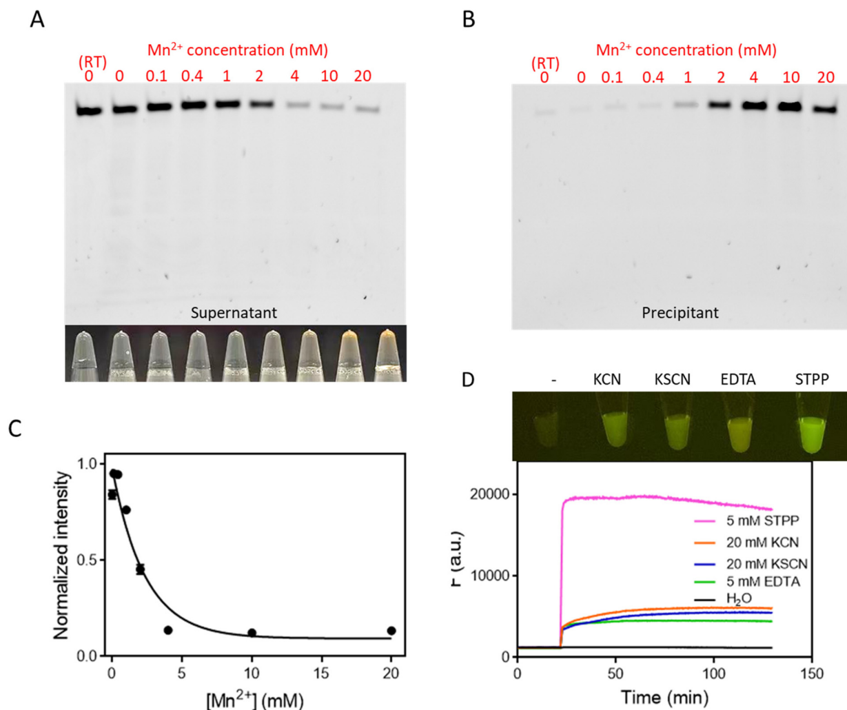
Fig. 4 Gel micrographs showing (A) the supernatants and (B) precipitates of the FAM-24mer (1 \mu M mixed with 3 \mu M nonlabeled DNA of the same sequence) mixed with different concentrations of Mn^{2+} at 95 ^{\circ} C for 3 h. A photograph of the samples is also shown in (A). (C) Quantification of the bands in (A). (D) Kinetics of fluorescence enhancement of the Mn/FAM-24mer by adding various metal binding ligands. A photograph of the samples at 470 nm excitation is also shown.
