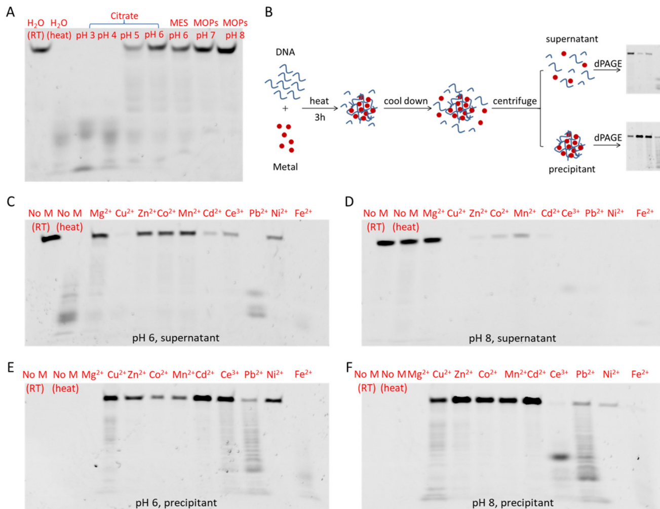
Fig. 1 (A) FAM-24mer (1 \mu M) incubated in buffers of different pH values at 95 ^{\circ} C for 3 h. The pH was adjusted using 50 mM buffer. (B) A scheme showing the experimental method. The gel micrographs of the FAM-24mer DNA mix with 4 mM different metal ions at 95 ^{\circ} C for 3 h in 5 mM (C and E) pH 6 MES buffer and (D and F) pH 8 MOPS buffer for the supernatants (C and D) and washed precipitates (E and F). The DNA concentration was 1 \mu M FAM-24mer mixed with 3 \mu M non-labeled DNA of the same sequence.
