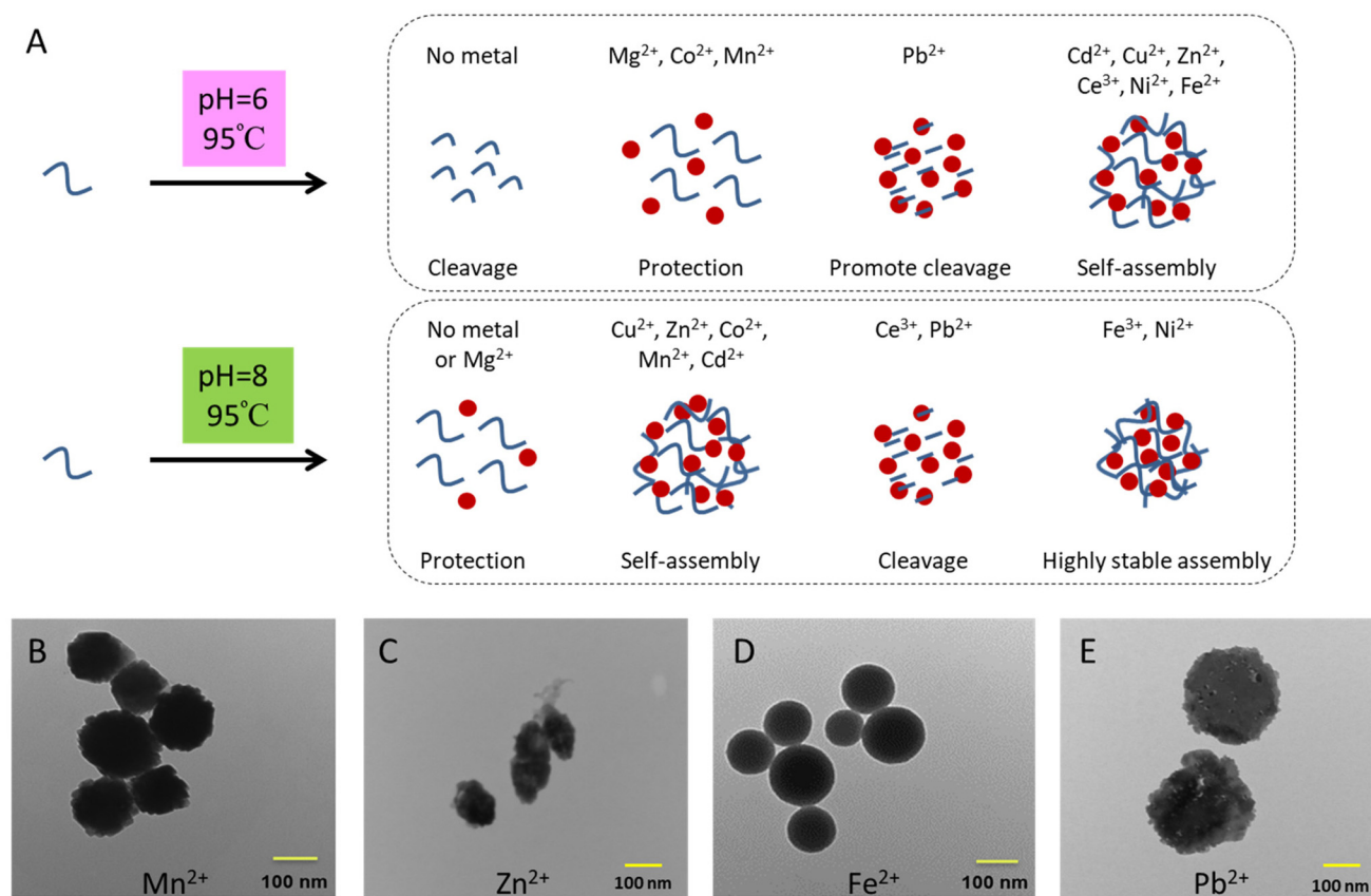
Fig. 2 (A) Classification of the effects of metal ions by incubating them with the DNA at 95 °C for 3 h at pH 6 and pH 8. TEM micrographs of nanoparticles formed by the 24-mer DNA and (B) Mn 2+ , (C) Zn 2+ , (D) Fe 2+ , and (E) Pb 2+ . The Fe 2+ NPs were prepared in water and the rest were prepared in 5 mM MOPS buffer at pH 8.
