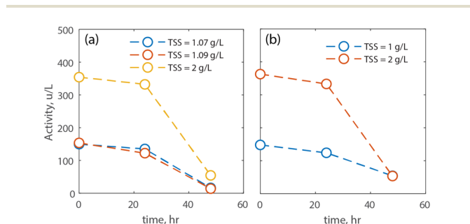
Fig. 12 Evolution of the activity of CA within the microalgae at (a) 25 °C and (b) 40 °C. CA was added to the system through different amounts of microalgae expressed as total suspended solids (TSS).
