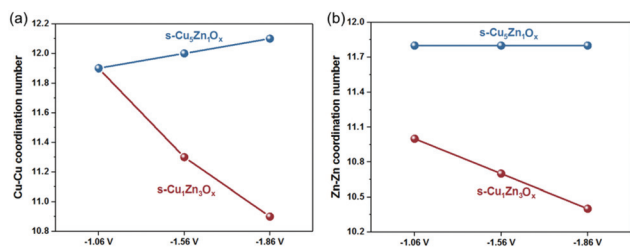
Fig. 6 Coordination number of the (a) Cu–Cu path and (b) Zn–Zn path as a function of potential for s\text{-Cu}_1\text{Zn}_3\text{O}_x and s\text{-Cu}_5\text{Zn}_1\text{O}_x .
