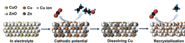
Fig. 7 Schematic process of the reconstruction of Cu sites during the \text{CO}_2\text{RR} .
