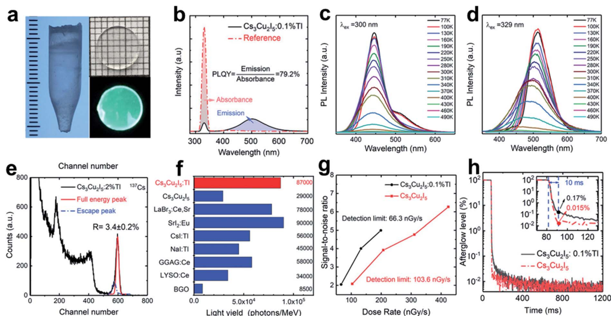
Fig. 9 (a) A \text{Cs}_3\text{Cu}_2\text{I}_5:\text{Tl}^+ crystal ingot grown in 7 mm diameter as well as a 1 mm thick panel under natural (up) and UV light (down). (b) PLQY profile of the 0.1% \text{Tl}^+ -doped- \text{Cs}_3\text{Cu}_2\text{I}_5 single crystal. (c and d) Temperature dependent photoluminescence spectra for 0.1% \text{Tl}^+ -doped- \text{Cs}_3\text{Cu}_2\text{I}_5 (77–490 K): (c) STE and (d) \text{Tl}^+ -centre emission respectively. (e) Pulse height profile of 2% \text{Tl}^+ -doped \text{Cs}_3\text{Cu}_2\text{I}_5 obtained from ^{137}\text{Cs} radiation source. (f) Comparisons in absolute LY between \text{Tl}^+ -doped and pure \text{Cs}_3\text{Cu}_2\text{I}_5 , and other typical scintillation materials. (g) Comparison in SNR as a function of X-ray dose rate for 0.1% \text{Tl}^+ -doped and pure \text{Cs}_3\text{Cu}_2\text{I}_5 . (h) Afterglow curves for 0.1% \text{Tl}^+ -doped and pure \text{Cs}_3\text{Cu}_2\text{I}_5 . 112 Copyright 2021 Wiley-VCH.
