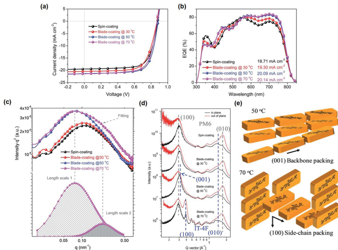
Fig. 15 (a) J - V curves, (b) EQE spectra, (c) RSoXS profiles, and (d) GIWAXS line profiles of PM6:IT-4F devices based on spin coating and blade coating at 30, 50 and 70 °C. (e) The schematics of molecular packing for IT-4F molecules in the blend films prepared by blade-coating at 50 and 70 °C. Adapted with permission. 123 Copyright 2019, The Royal Society of Chemistry.
