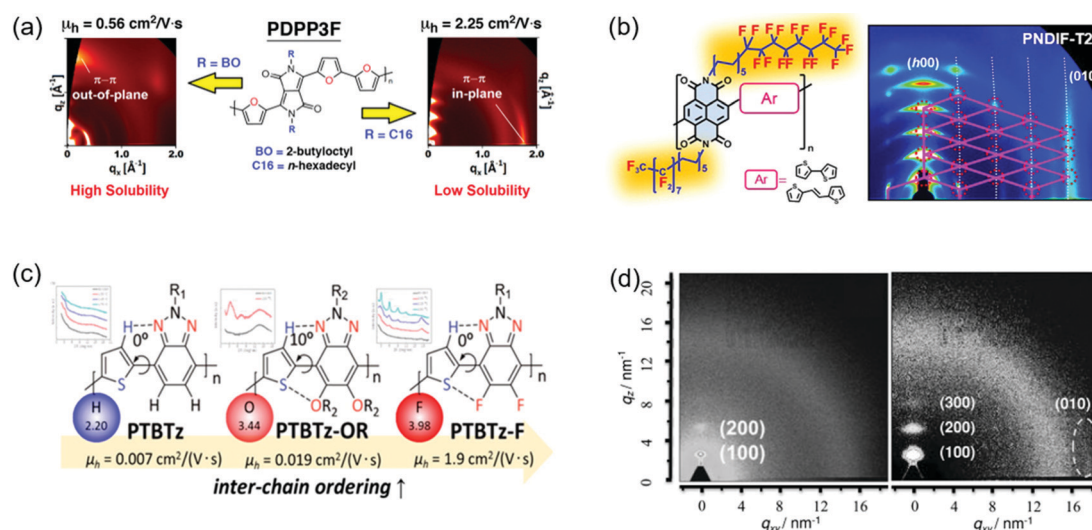
Fig. 12 Improving the crystallinity of CPs by side chain engineering and fluorine substitution. (a) GIXRD patterns of PDPP3F containing different side chains. Reproduced with permission. 167 Copyright 2013, American Chemical Society. (b) The molecular structures and GIXRD patterns of NDI-based polymers containing semifluorinated side chains. Reproduced with permission. 163 Copyright 2016, American Chemical Society. (c) The molecular structures of benzotriazole-based polymers containing different substituted atoms. Reproduced with permission. 171 Copyright 2014, American Chemical Society. (d) 2D GIWAXS of the annealed films of PDPP-TVt (left) and PDPP-4FTVt (right). Reproduced with permission. 172 Copyright 2015, Wiley-VCH.
