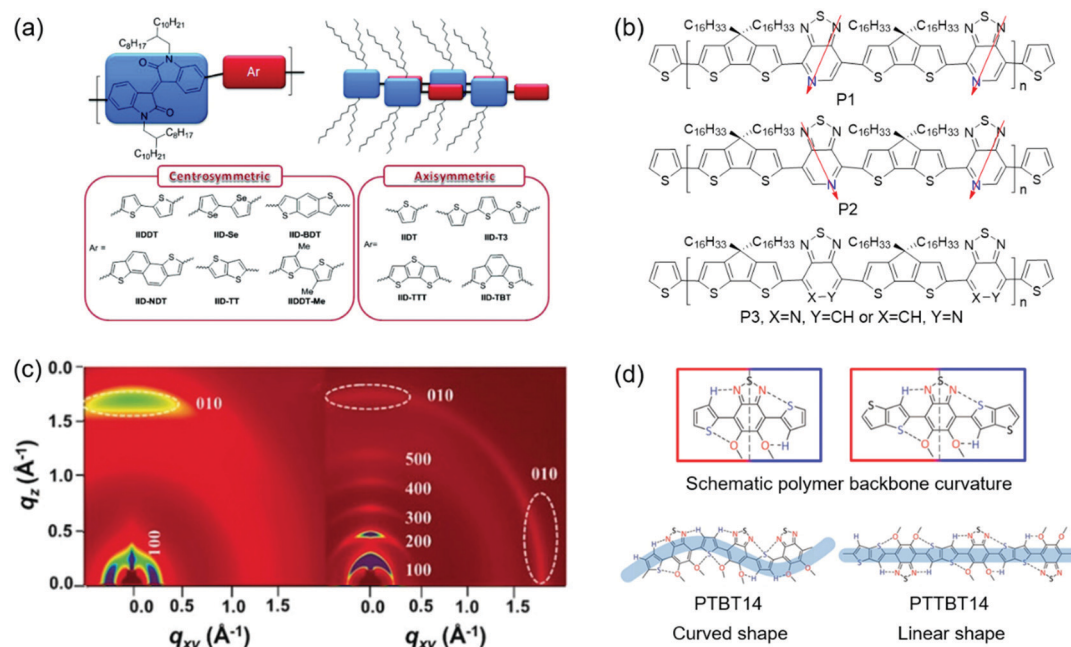
Fig. 11 Improving the crystallinity of CPs by molecular geometry modulation. (a) The molecular structures of isoidindigo-based polymers containing centrosymmetric and axisymmetric units. Reproduced with permission. 152 Copyright 2012, American Chemical Society. (b) The molecular structures of regioregular polymers (P1 and P2) and a regiorandom polymer (P3). (c) 2D-GIWAXS of s-BTI2-FT (left) and f-BTI2-FT (right). Reproduced with permission. 158 Copyright 2017, Wiley-VCH. (d) The molecular structures of two polymers (PTBT14 and PTTBT14) with different backbone curvatures. Reproduced with permission. 159 Copyright 2014, American Chemical Society.
